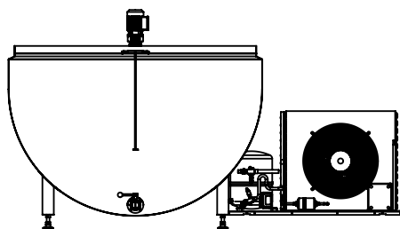
VISTA FRONTAL
